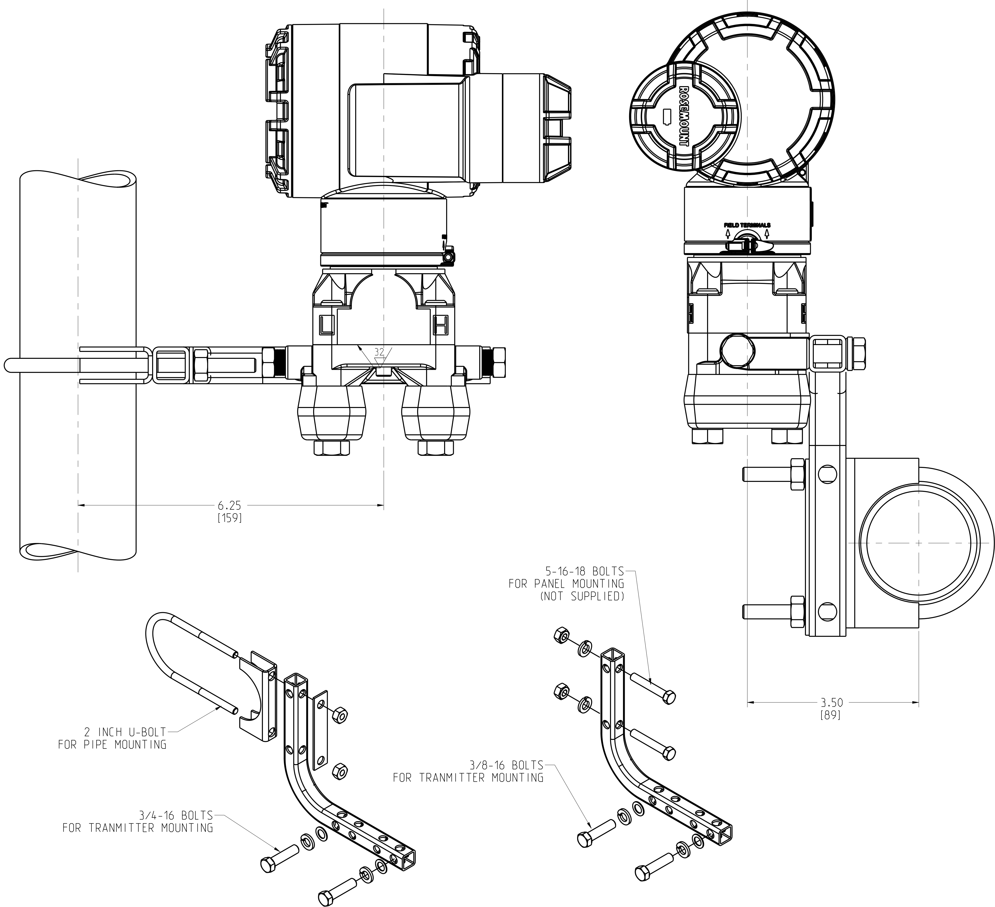
PIPE MOUNTING
