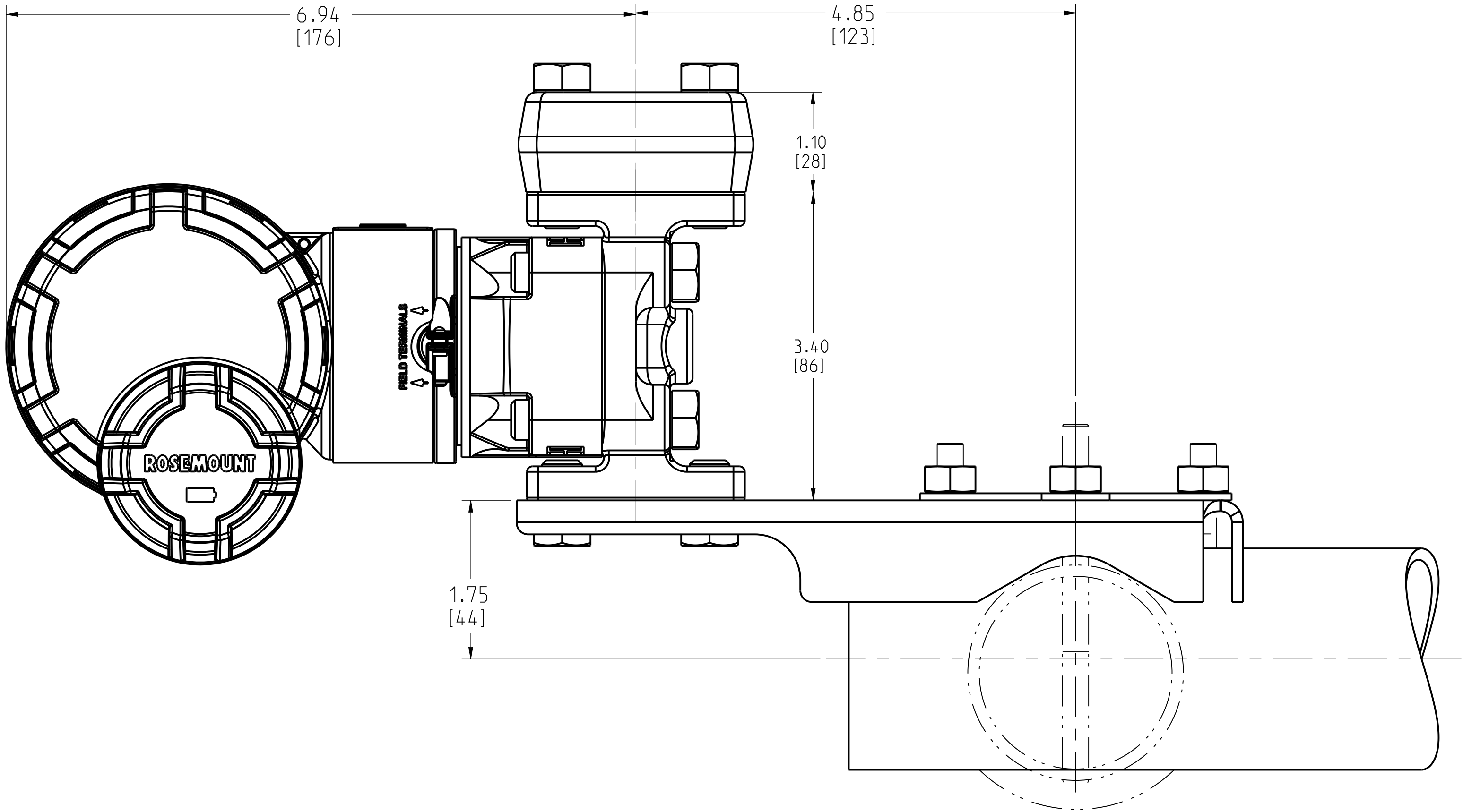
PIPE MOUNTING
