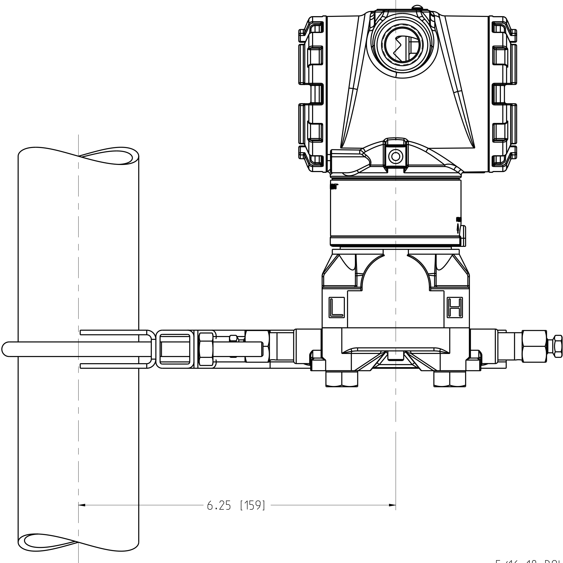
PIPE MOUNTING
